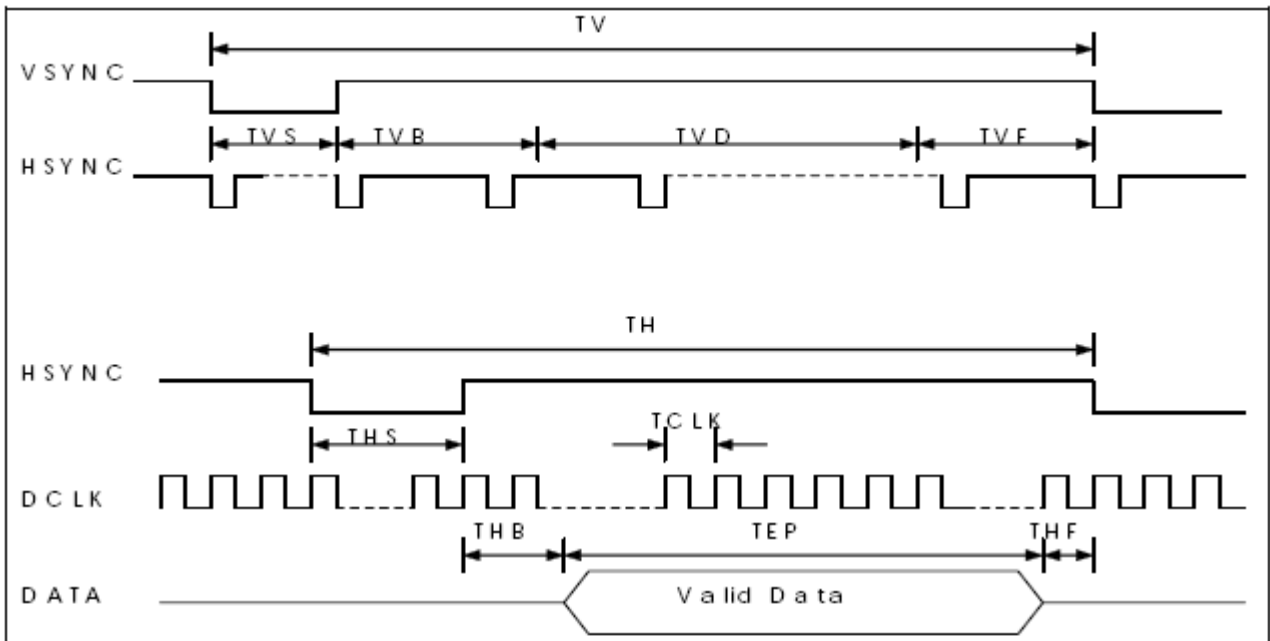
Figure 7 IHS and IVS timing waveforms
